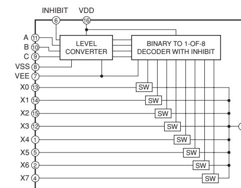
IC111, 112: TC74HC4051AP Analog Multiplexer/Demultiplexer
