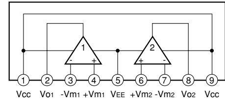
IC202: μPC4570HA Dual OP-Amp
