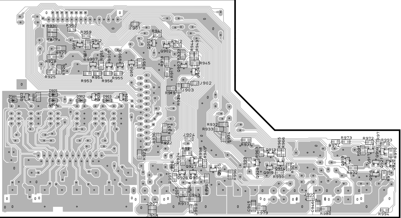
VIDEO (2) P. C. B. (Surface Mount Device)
