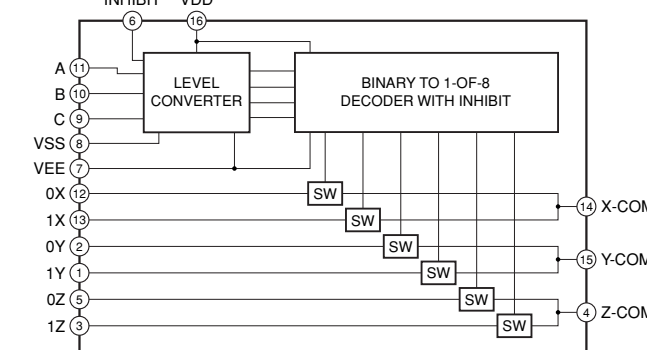
IC113: TC74HC4053AP Analog Multiplexer/Demultiplexer
