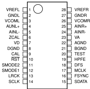
IC9: AK5383-VS (DSP P.C.B.) 24 bit 2ch A/D Converter
