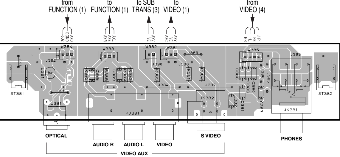
VIDEO (3) P. C. B. (Lead Type Device)
