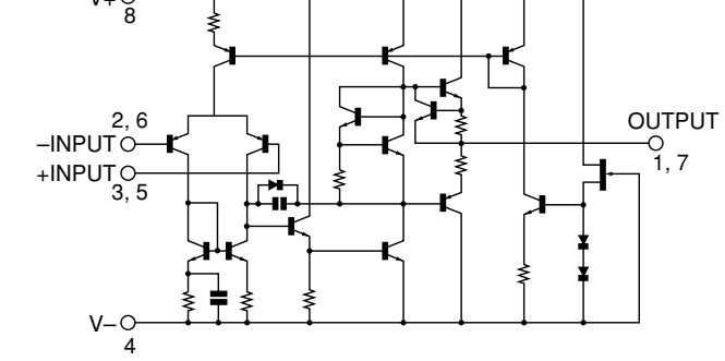
IC203: NJM4556AL Dual OP-Amp
