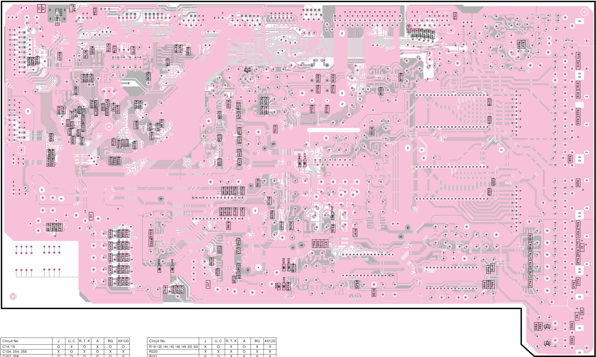
FUNCTION (1) P. C. B. (Surface Mount Device)
